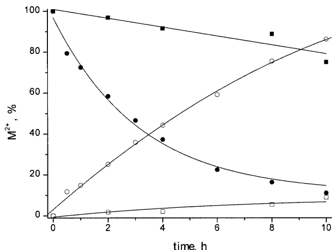
Figure 3. Mol percentage of \text{Hg}^{2+} (circles) and \text{Pb}^{2+} (squares) vs. time in the source phase (filled symbols) and receiving phase (open symbols) in the simultaneous transport; [\text{bis-}p\text{ODET}] = 1 \times 10^{-3} \text{ M} in chloroform; [\text{PbCl}_2] = [\text{HgCl}_2] = 2.5 \times 10^{-3} \text{ M} in 0.15 M acetate buffer, pH = 4.68; receiving phase: 0.5 M HCl, pH = 0.3; T = 25^\circ\text{C}
