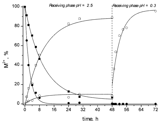
Figure 2. Mol percentages of \text{Hg}^{2+} (circles) and \text{Cd}^{2+} (squares) vs. time in the source phase (filled symbols) and receiving phase (open symbols) in simultaneous transport; [\text{bis-}p\text{ODET}] = 2 \times 10^{-3} \text{ M} in chloroform; [\text{CdCl}_2] = [\text{HgCl}_2] = 2.5 \times 10^{-3} \text{ M} in 0.15 M acetate buffer, pH = 4.68; T = 25^\circ\text{C} ; see text for the experimental procedure
