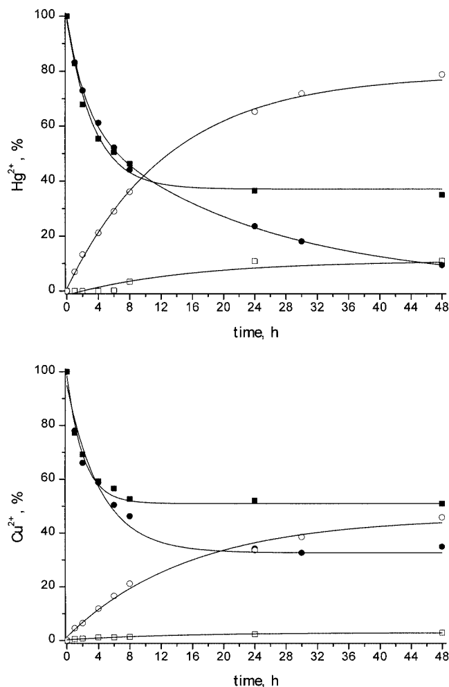
Figure 1. Mol percentages of Hg^{2+} (top) and Cu^{2+} (bottom) vs. time in the source phase (filled symbols) and receiving phase (open symbols) with 3.2 \times 10^{-3} M HCl, pH = 2.5 (squares) and 0.5 M HCl, pH = 0.3 (circles) as receiving phase; [bis- p ODET] = 1 \times 10^{-3} M in chloroform; [MCl_2] = 5 \times 10^{-3} M in 0.15 M acetate buffer, pH = 4.68; T = 25 °C
