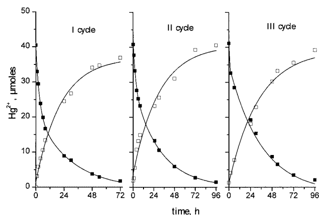
Figure 4. \mu moles of Hg^{2+} in the source phase (filled squares) and receiving phase (open squares) in three consecutive cycles; [bis- p O-DET] = 1 \times 10^{-3} M in chloroform; [ HgCl_2 ] = 5 \times 10^{-3} M in 0.15 M acetate buffer, pH = 4.68; receiving phase: 0.5 M HCl, pH = 0.3; T = 25 °C.
